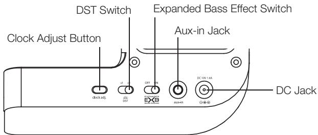
Back Panel
